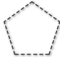
Area_Polygon
