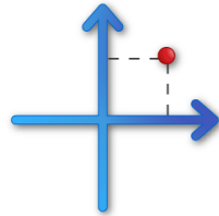
CoordinateSystem_Cartesian_2D
