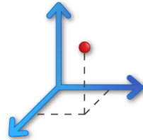
CoordinateSystem_Cartesian_3D
