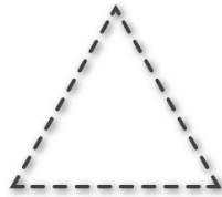
Area_Triangle
