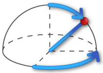
CoordinateSystem_Spherical
