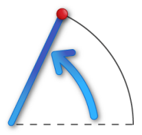
CoordinateSystem_Polar
