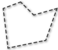
Area_CustomPolygon
